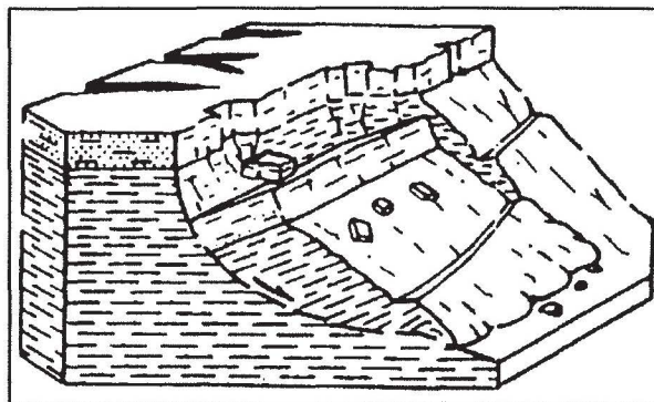
4. Rotational slide
