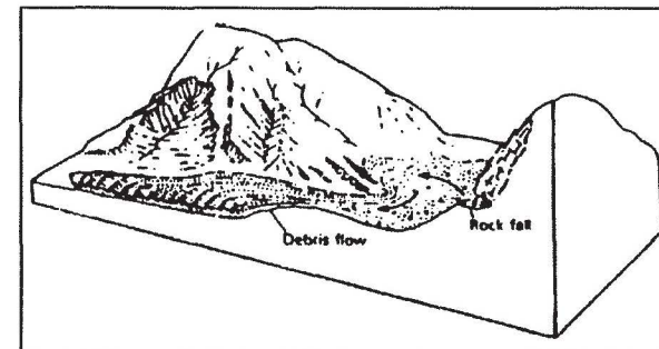
5. Debris flow
